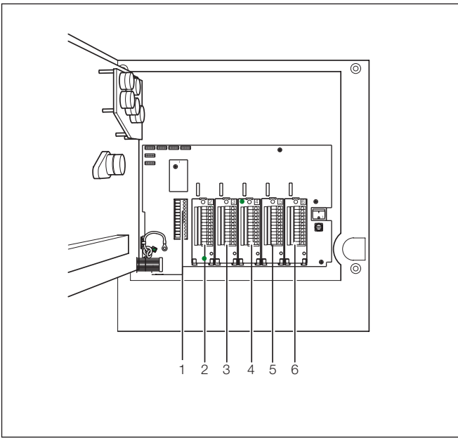
Module Positions
