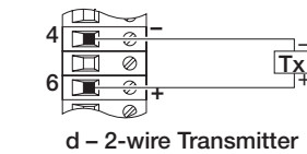
d – 2-wire Transmitter
