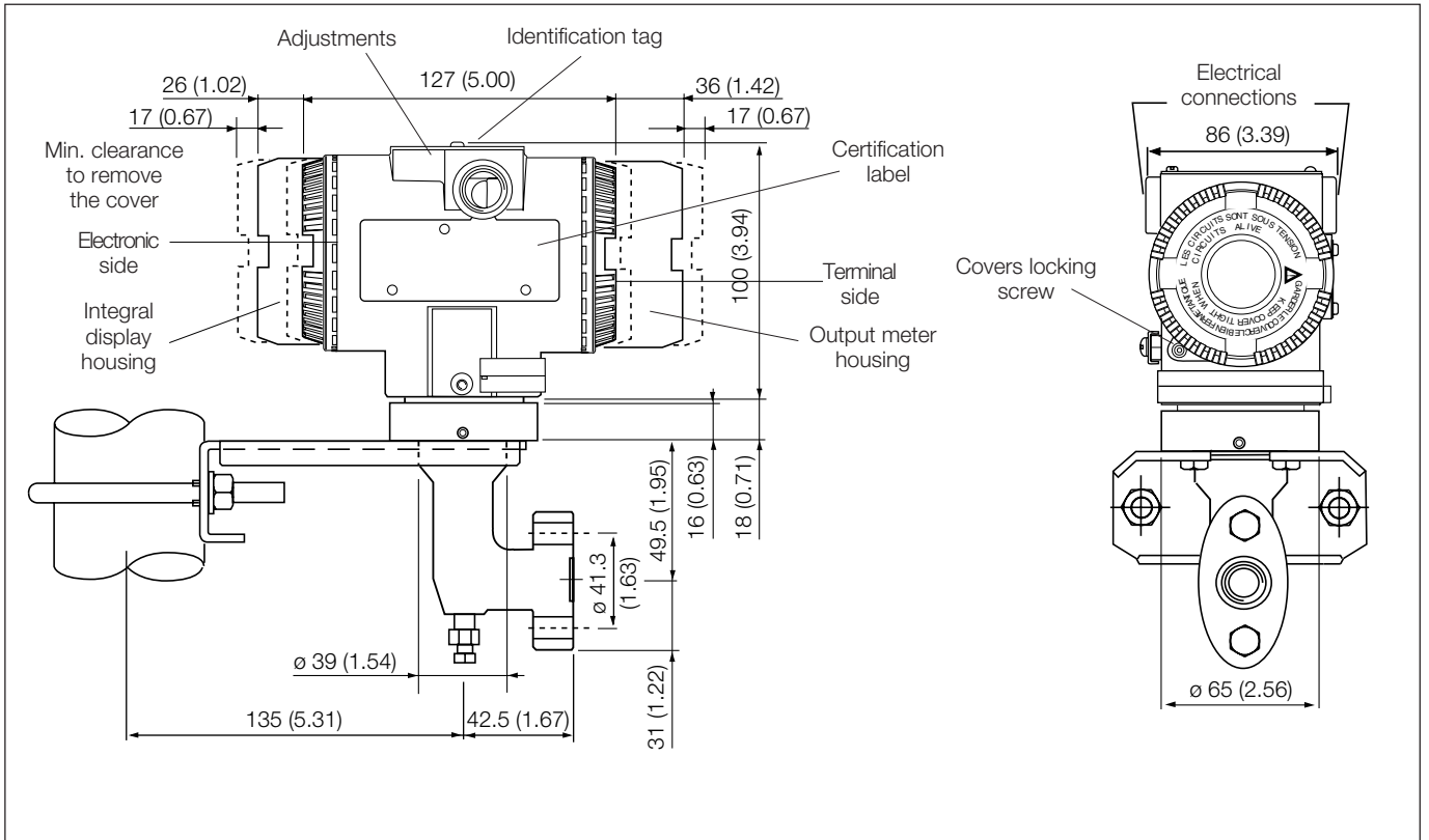
Adapter angle (90°) entry connection (1/16in - 20 UNF drilling)
