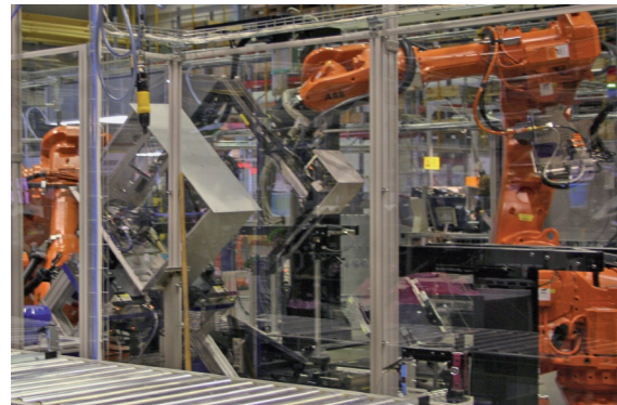
RobotWare-Dispense in a MultiMove system in the robot factory in Västerås.
