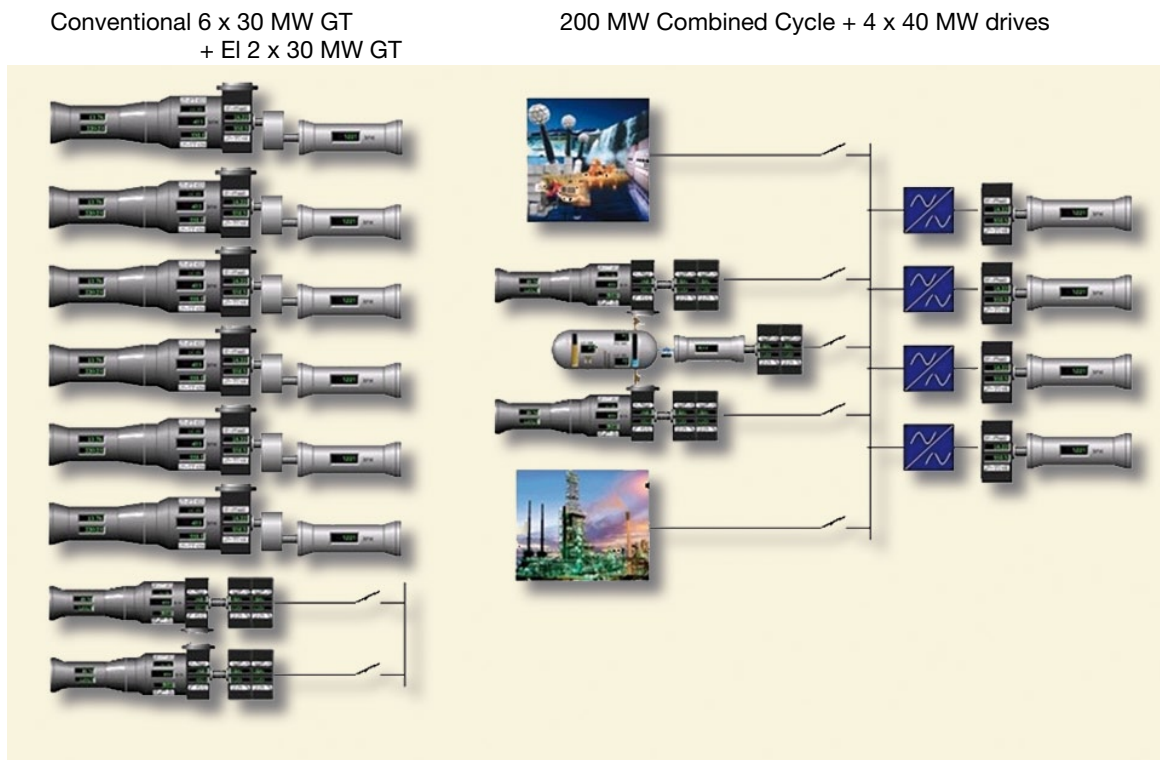
Figure 2 Reference system gas turbines vs. all electric
