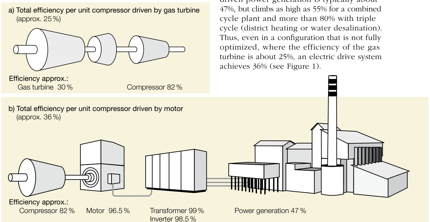
Figure 1 Efficiency per unit of centrifugal compressor driven by motor and gas turbine indicates total efficiency for motor and gas turbine driven systems, respectively
