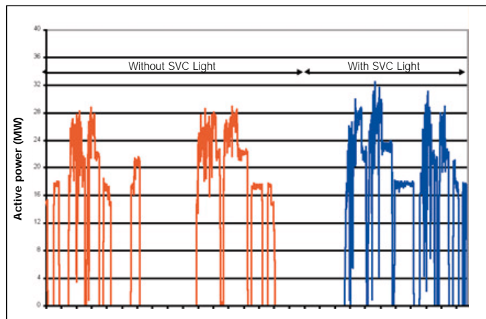
Active power into the EAF without and with dynamic compensation.
