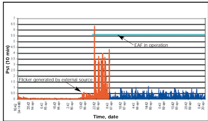
Flicker generation without and with SVC Light.
