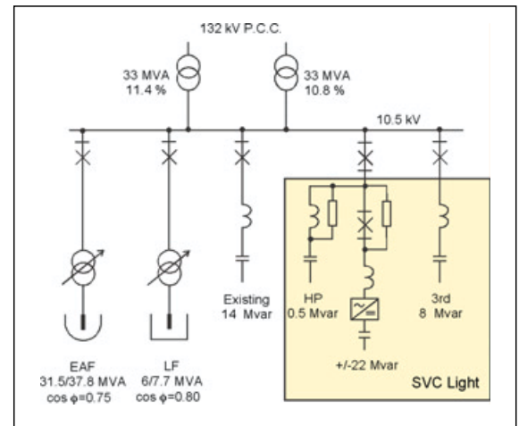
Single-line diagram
