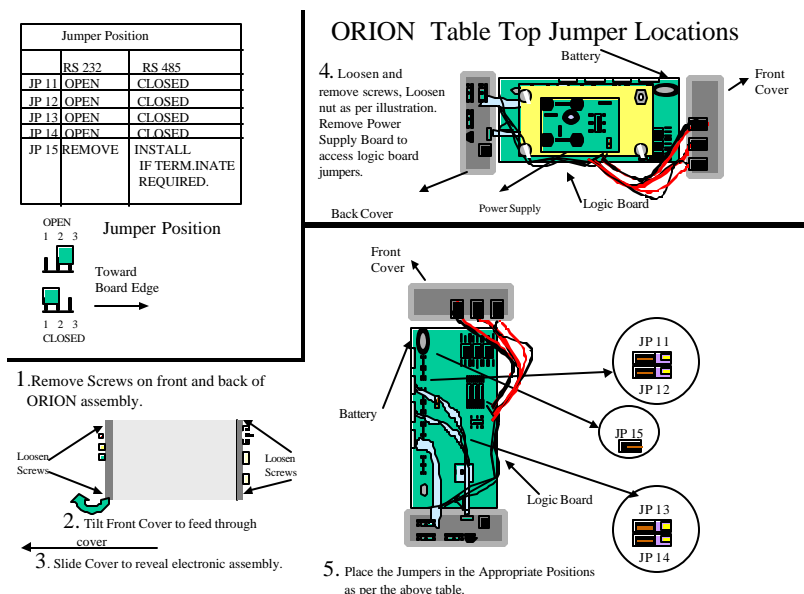
Figure 3A - Orion Table Top Jumper Locations
