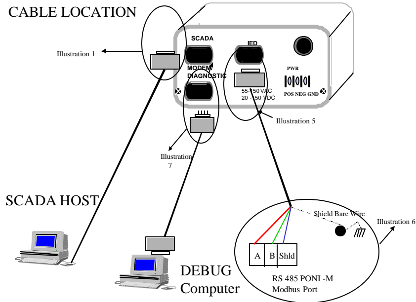
Figure 2A – Orion Table Top Cable Connection Diagram
