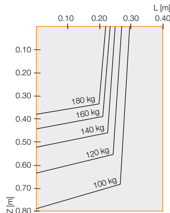
IRB 660 180/3.15
