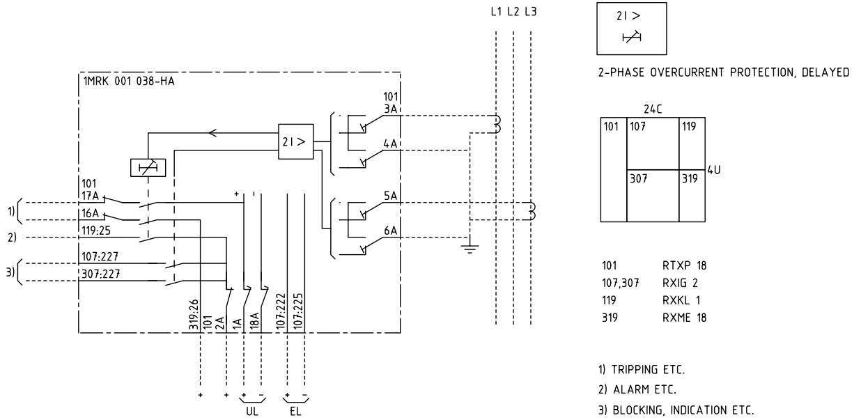
Fig. 3 Terminal diagram No. 1MRK 001 038-HAA for RAIG, 1MRK 001 037-HA
