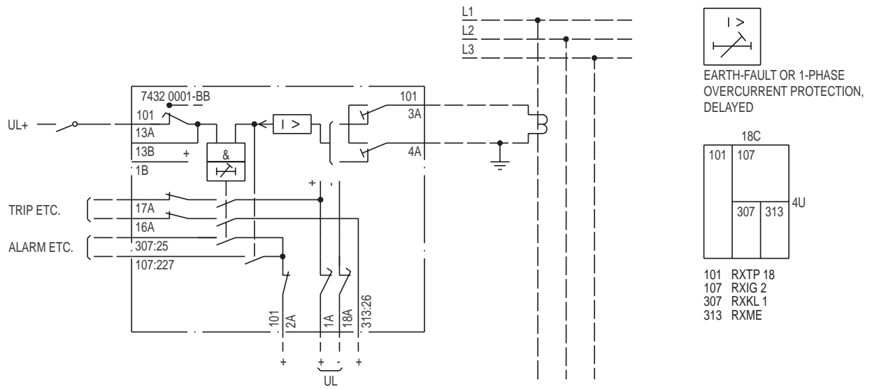
Fig. 5 Terminal diagram No. 7432 0001-BBA for RAIG, RK 651 100-BB
