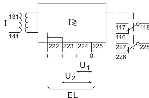
Fig. 2 Circuit diagram for RXIG 2
