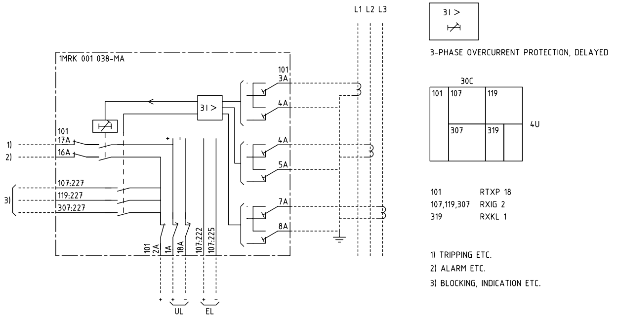
Fig. 4 Terminal diagram No. 1MRK 001 038-MAA for RAIG, 1MRK 001 037-MA
