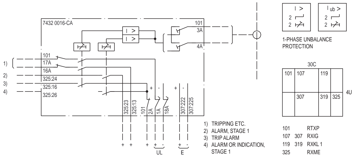
Fig. 6 Terminal diagram No. 7432 0016-CAA for RAIG, RK 651 116-CA
