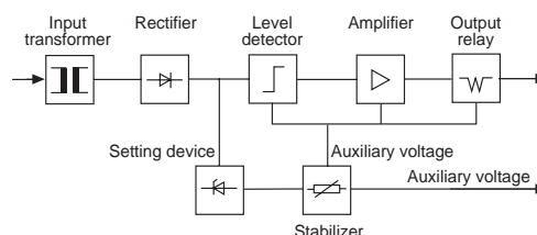
Fig. 1 Block diagram of RXIG
