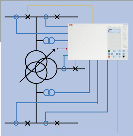
RET 670 ensures enhanced through-fault stability for multi-breaker arrangements
